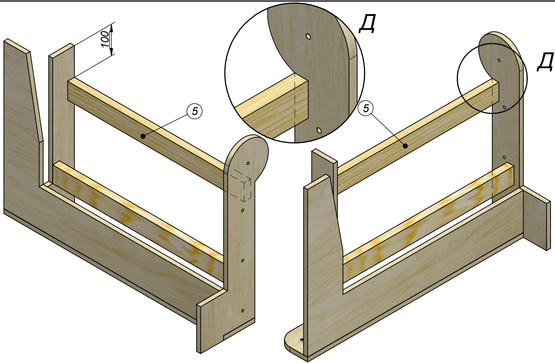
5. Wooden beam 60 x 25 x 650 - 1
